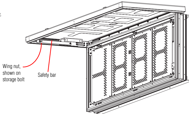
Inside view of the case, showing safety bar in stored position inside the door
