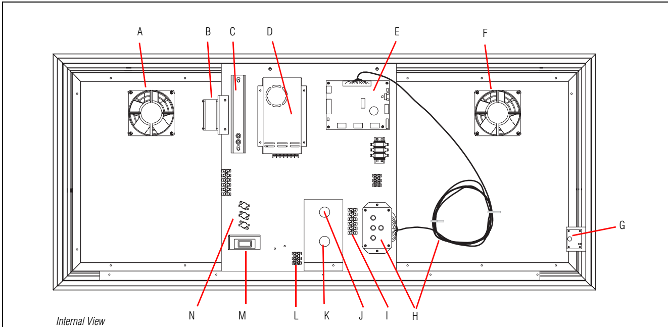
Internal View
